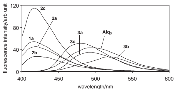
Figure 2. Fluorescence spectra of Al complexes in the solid state.
