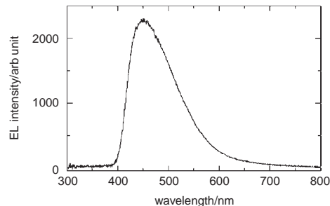
Figure 3. The emission spectrum of Al complex 1a .
