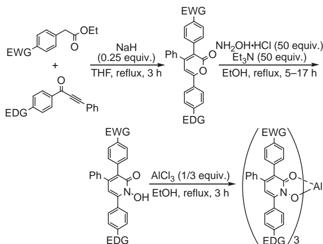
Scheme 1. Synthesis of aluminum complexes.
