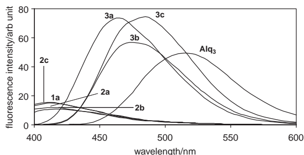
Figure 1. Fluorescence spectra of Al complexes in \text{CH}_2\text{Cl}_2 ( 1.0 \times 10^{-4} M).
